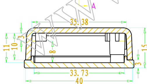
SEC B-B
